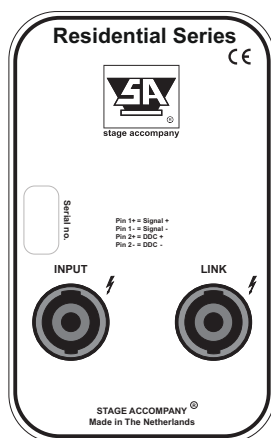
The RSB51 SpeakON NL4 connectors
