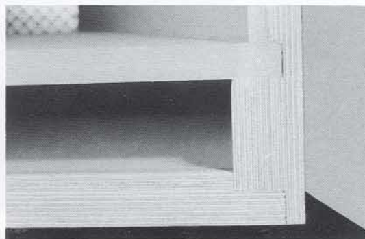
Typical panel joint construction of the 4512
