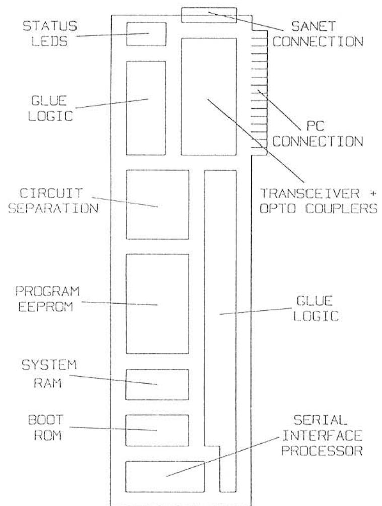
FIGURE 3. SANET CONTROLLER EXTENSION CARD.
